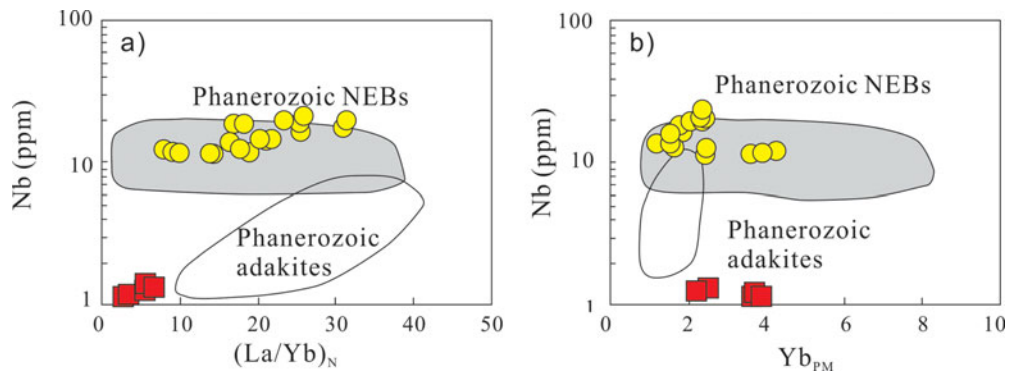
Figure 13. (Colour online) (a) (\text{La}/\text{Yb})_N and (b) \text{Yb}_{PM} v. Nb diagrams for the basalts from the Zhaheba area, indicating that G1 basalts have features of Nb-enriched basalts (NEBs).
